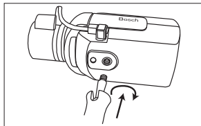
Figure 5.3 Mounting a camera
